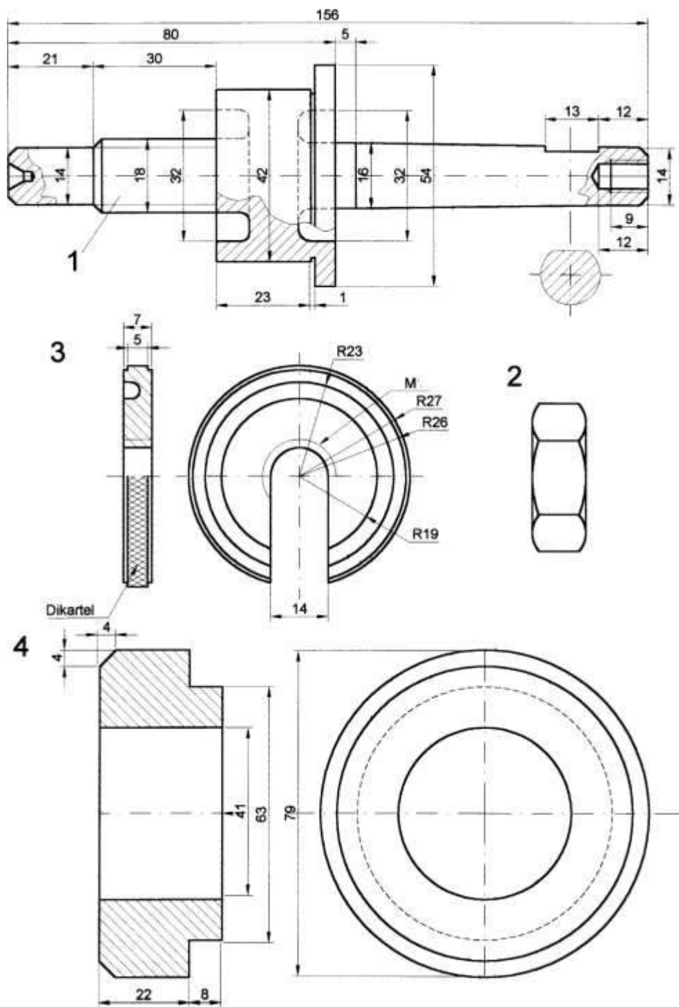
Gambar 6.8 (Detail Mandril)
