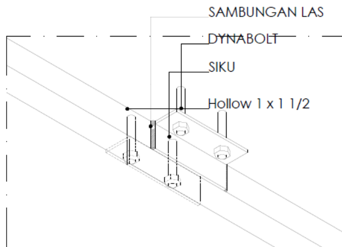
DETAIL A SKALA PROPORSIONAL
