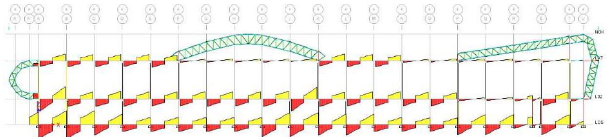
Gambar 4.3. Bidang Lintang Portal As 4 Akibat Beban Gempa Arah X
