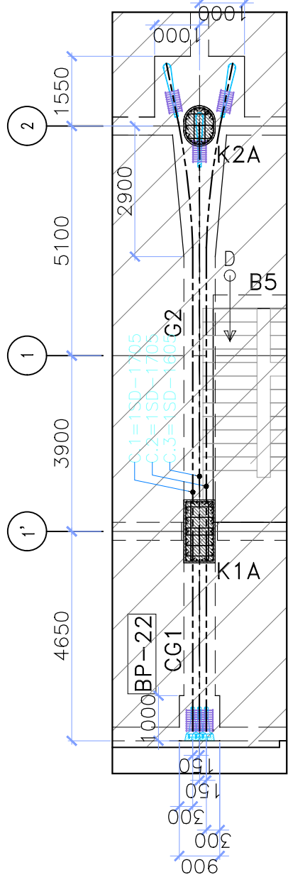
PLAN VIEW BP-22 (700x850/700)
