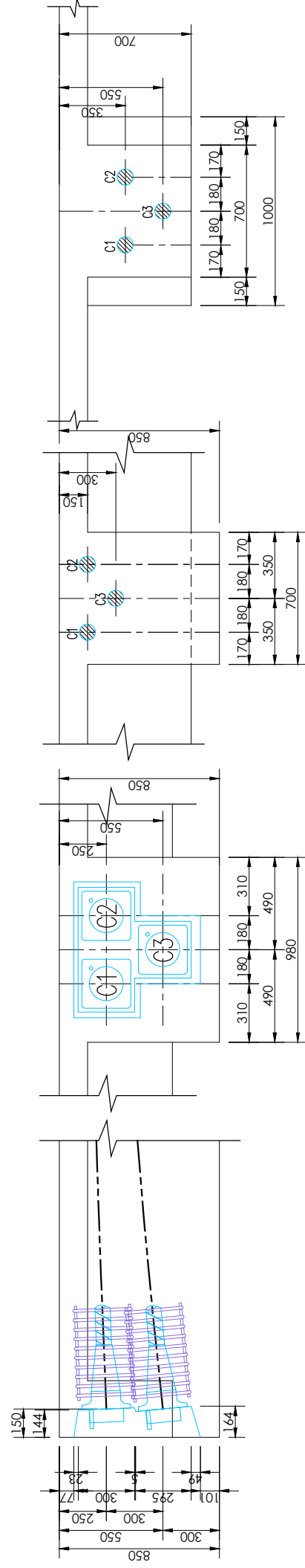
DETAIL - 1
