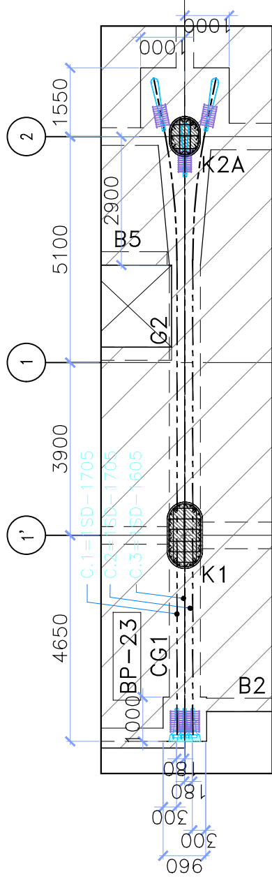
PLAN VIEW BP-23 (700x850/700)
