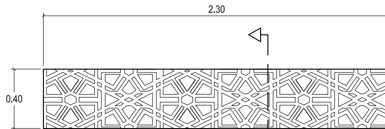
DETAIL 3 SCALE 1: 25
