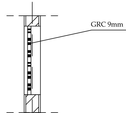
SECTION B SCALE 1: 25
