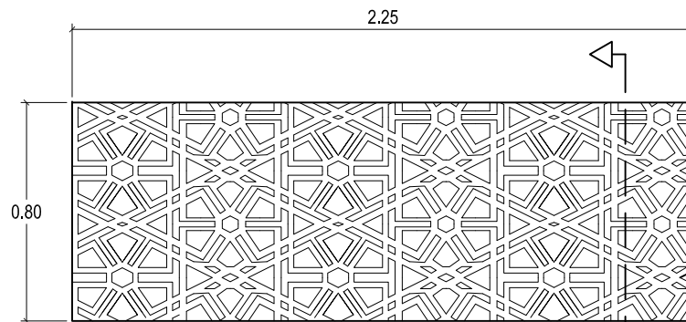
DETAIL SCALE 1: 25 2
