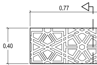
DETAIL SCALE 1: 25 1
