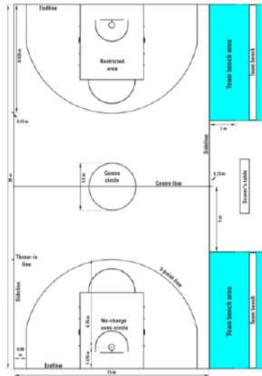
Gambar 2. Standar Lapangan Basket Sumber: FIBA Official Basketball Rules 2020
