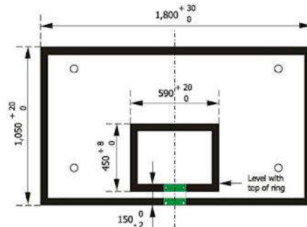
Gambar 5. Standar Ukuran Papan Pantul Sumber: FIBA Official Basketball Rules 2020
