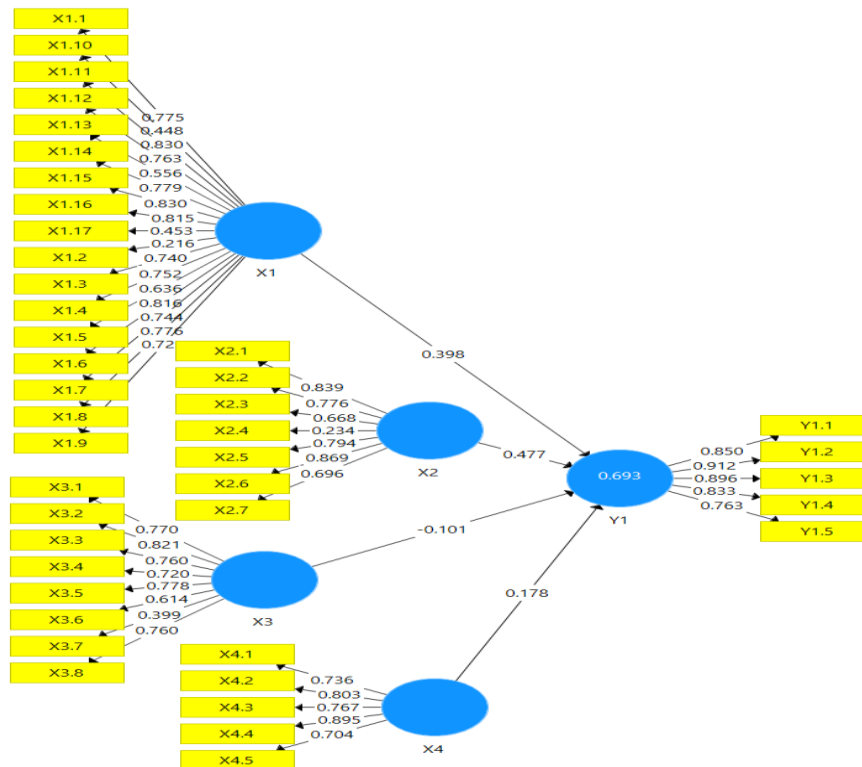
Gambar 2. Path modeling
