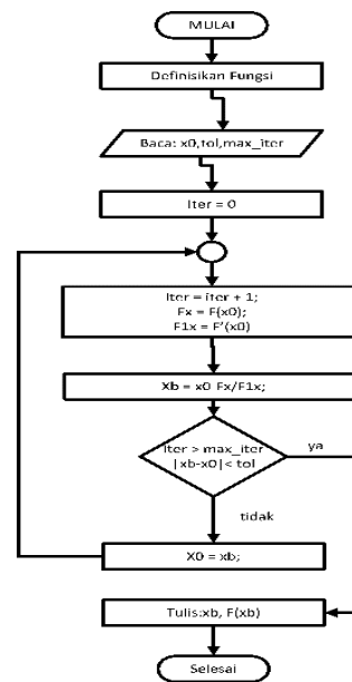
Gambar 8. Flowchart Algoritma Metode Newton Raphson
