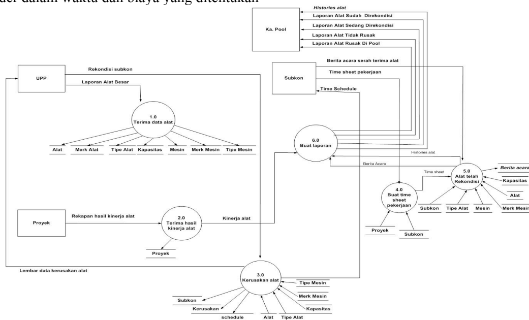
Gambar 1. Diagram Aliran Data Level 0
