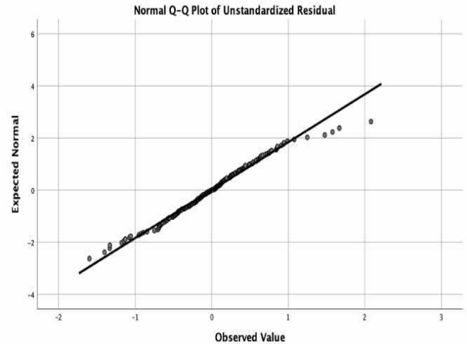
Figure 2 Normality test
