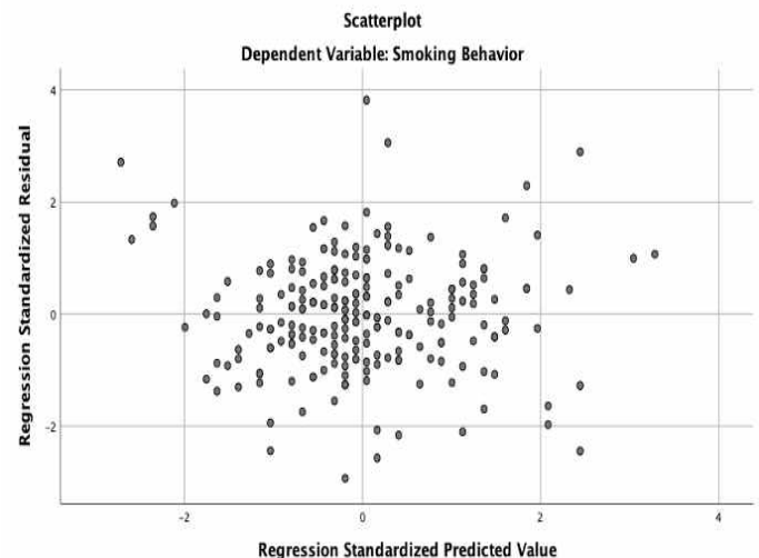
Figure 4 Scatterplot heteroscedasticity
