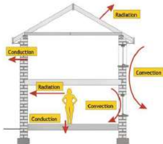
Figure 4. Building Heat Transfer (NN, 2009)
