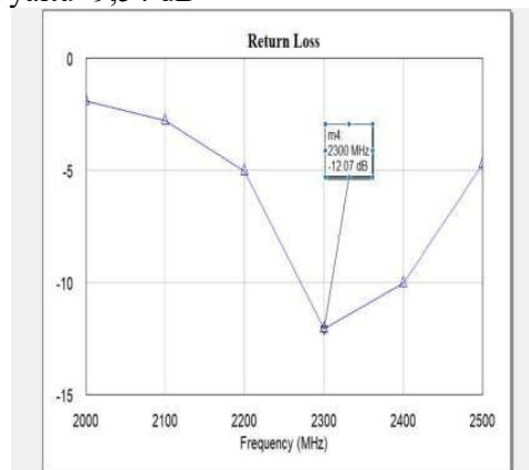
■ Gambar 8. Nilai Return Loss
