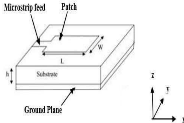
■ Gambar 3. Rectangular Patch
