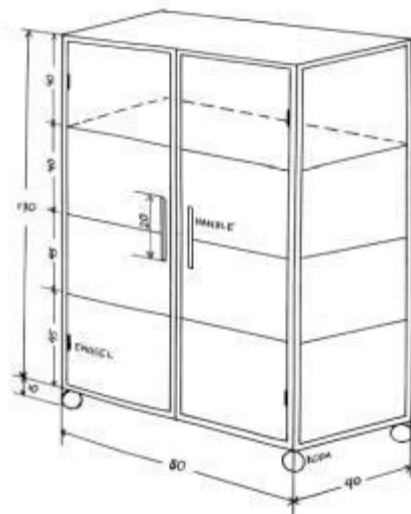
Gambar 4. Disain Lemari Inventaris Sumber: Sukania et al. (2020)
