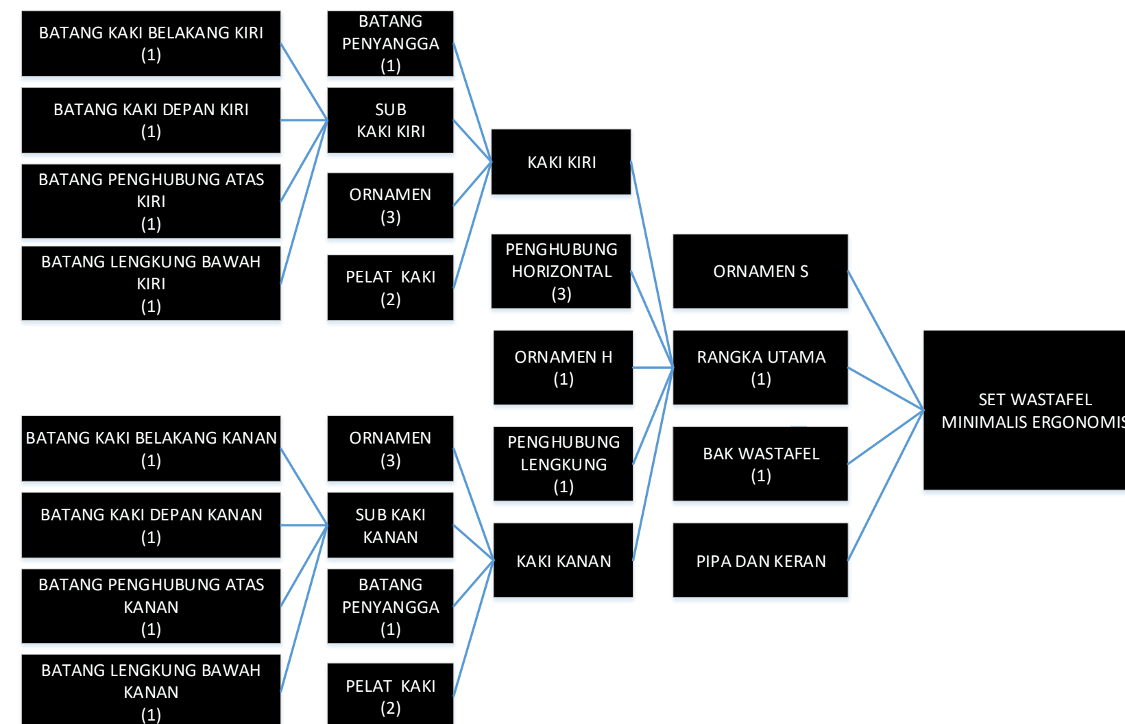
Gambar 2. Diagram Perakitan Wastafel Minimalis Ergonomis
