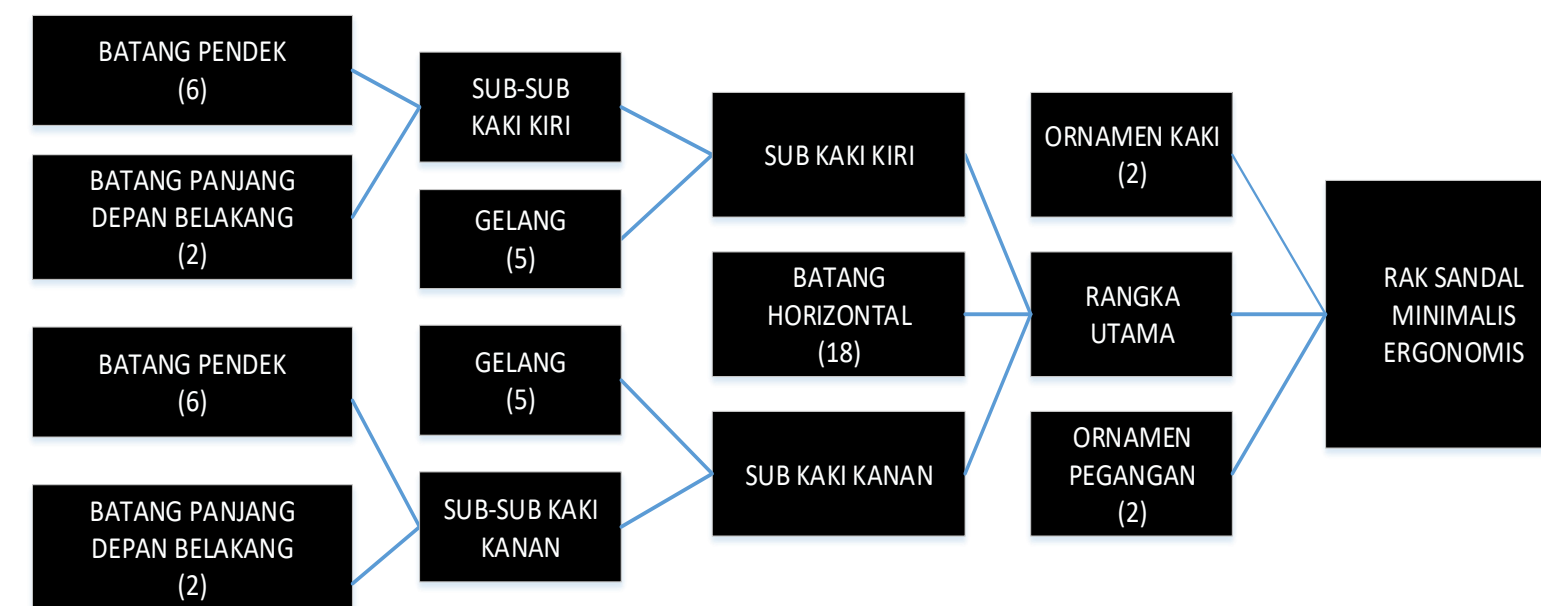
Gambar 2. Diagram Perakitan Rak Sandal Minimalis Ergonomis
