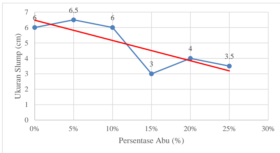
Gambar 4. Nilai workabilitas slump beton
