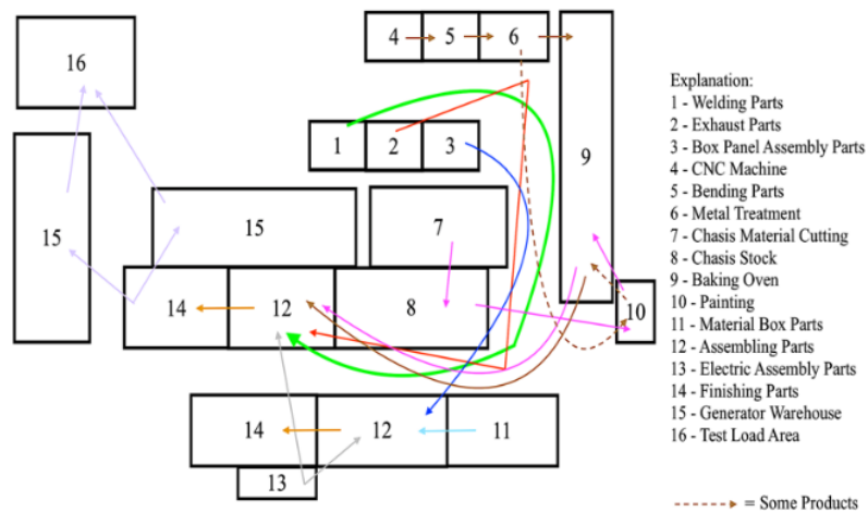
Figure 7. Initial Layout Flow Process
