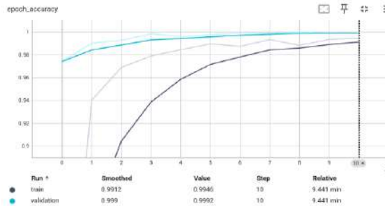
Gambar 8. Grafik akurasi training custom CNN
