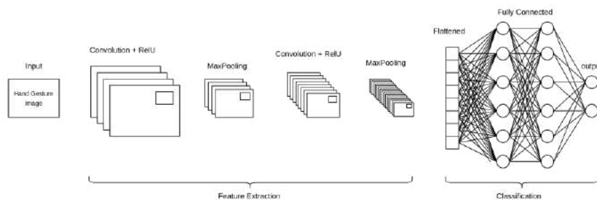
Gambar 6. Custom CNN
