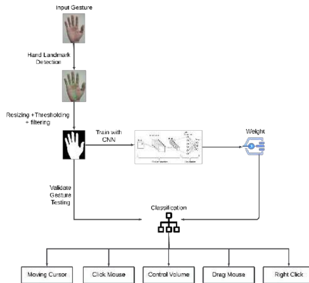
Gambar 2. Rancangan Sistem Virtual Mouse
