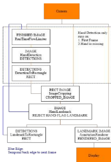
Gambar 4. Hand Landmark Detection Graph [8]
