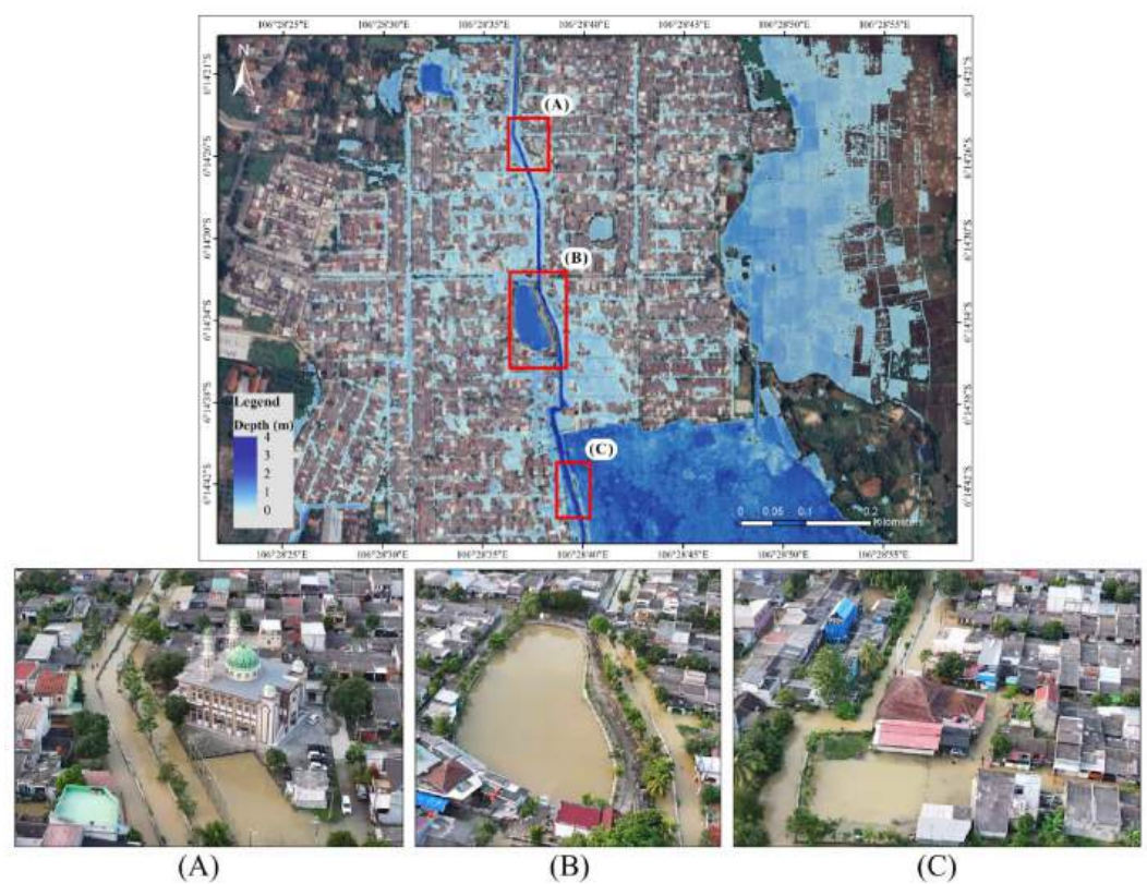
Figure 12. Flood event calibration point.
