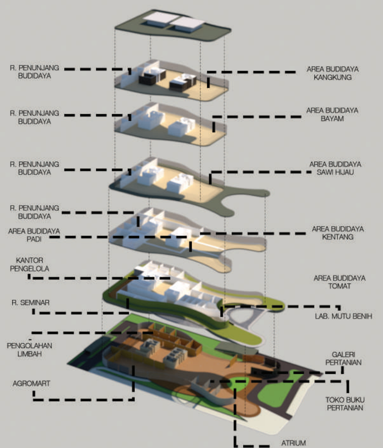
EXPLODED PLAN
