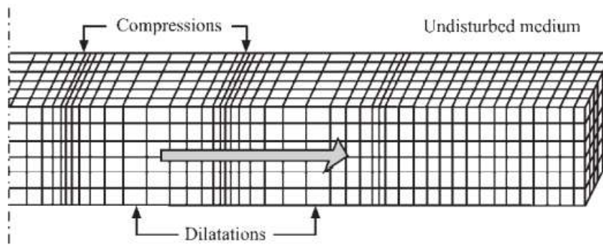
Gambar 6. Gelombang longitudinal (P-Wave) (Elnashai & Sarno, 2008)
