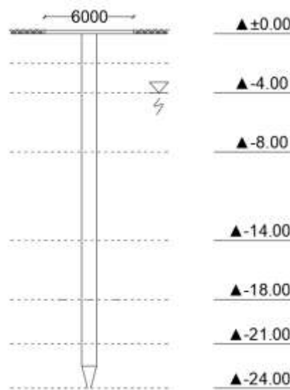
Gambar 7. Sketsa sistem fondasi suspended
