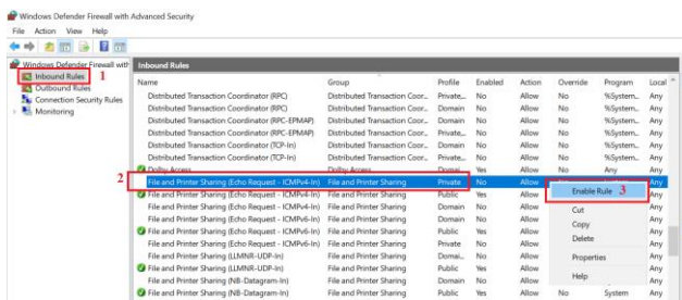
Gambar. 9 Konfigurasi Pengaktifan Aturan File and Printer Sharing (Echo Request ICMPv4-In)
