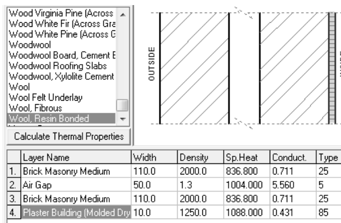
Gambar.7 Potongan Dinding Double Brick Cavity Plaster
