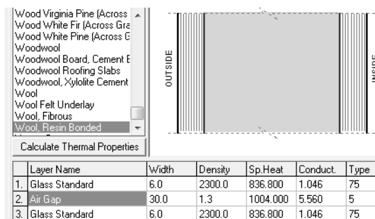
Gambar.9 Potongan Kaca Jendela Double Glazed Low-E Aluminium Frame Sumber: Ecotect Analysis 2011
