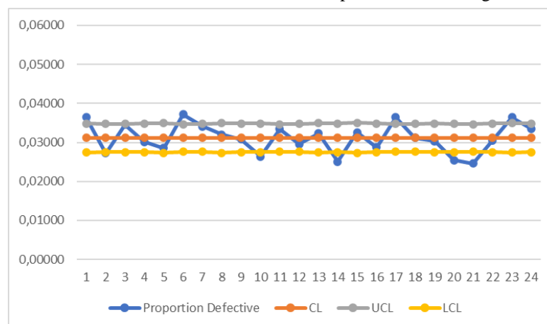
Figure 6. P Chart
