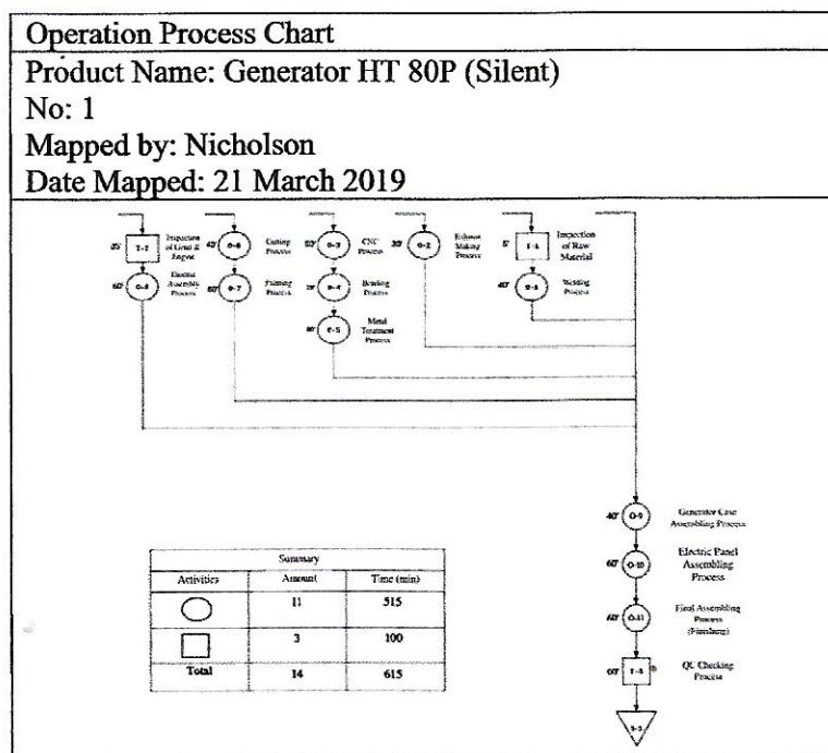
Figure 2. OPC Manufacture of Generator HT 80P
