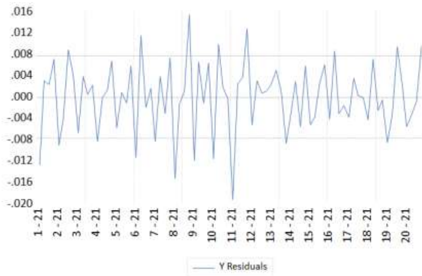
Gambar 2. Heterocedasticity Test Sumber: Ouput Eviews
