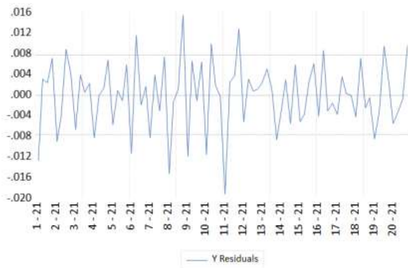
Gambar 2. Heterocedasticity Test
