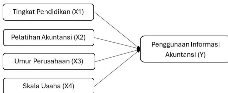
Gambar 1. Model Penelitian
