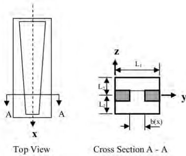
Figure 2. Model geometric of the artificial basilar membrane prototype
