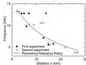
Figure 5. Resonance frequency along of the ABM at 75 dB - first experiment and 80 dB - second experiment
