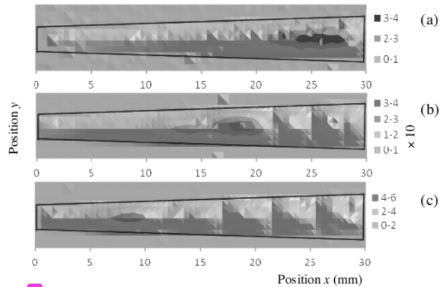
Figure 5 Contour map of the vibrating amplitude of the ABMP membrane at f = (a) 6 kHz, (b) 9 kHz, and (c) 12.8 kHz.
