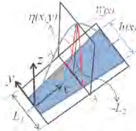
Figure 3 Description of the envelope curve W(x) and a single mode of the vibrating amplitude in y direction \eta(x, y) .
