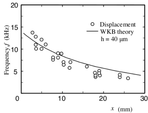
Figure 7 Relationship between the length of the membrane ( x ) and the local resonance frequency ( f ) at 5 dB.
